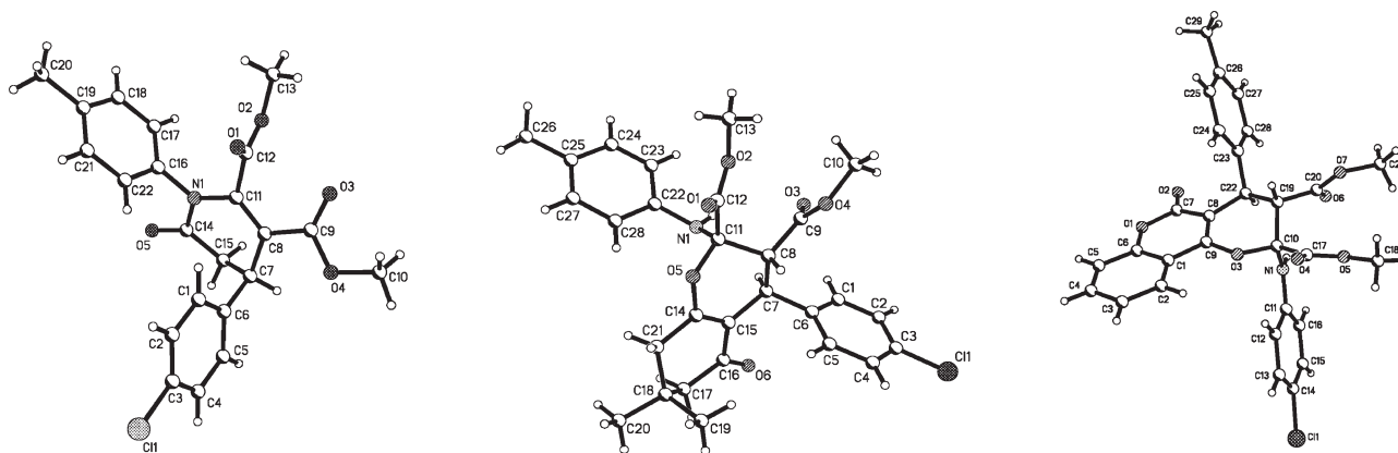
Figure 1. Molecular structure of 3,4-dihydropyridin-2(1H)-one 1c and 3,4-dihydro-2H-pyrans 2f , 4b .
